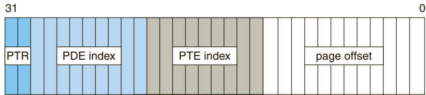
Figure 17.4 Virtual-to-physical address translation on IA-32.
