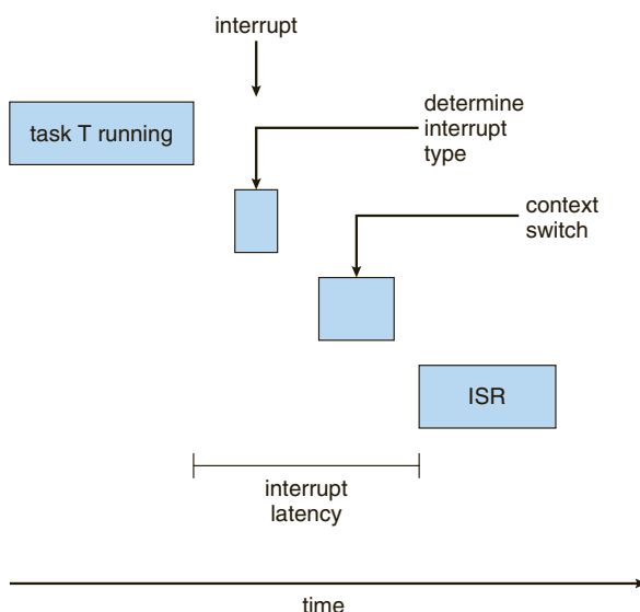
Figure 5.13 Interrupt latency.
