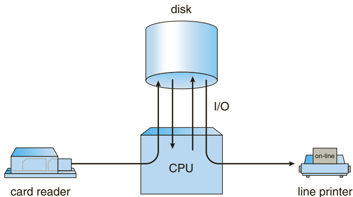
Figure 18.5 Spooling.
