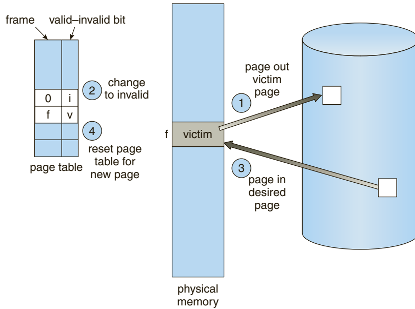
Figure 9.10 Page replacement.
