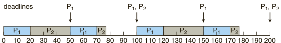
Figure 5.17 Rate-monotonic scheduling.
