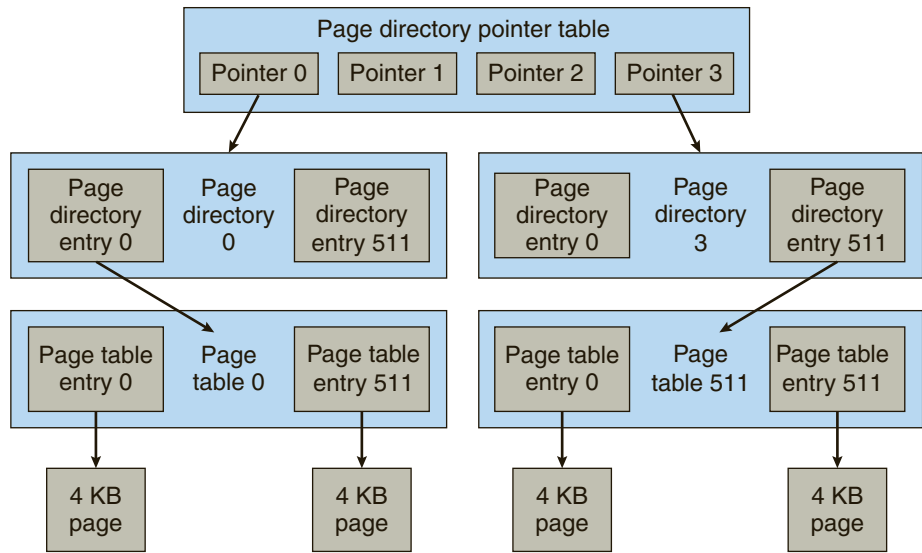
Figure 17.3 Page-table layout.
