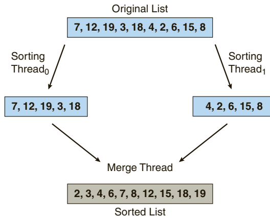
Figure 4.20 Multithreaded sorting.
