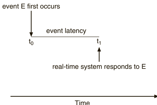
Figure 5.12 Event latency.
