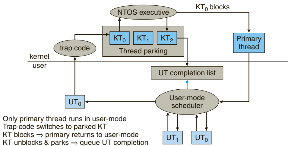
Figure 17.11 User-mode scheduling.
