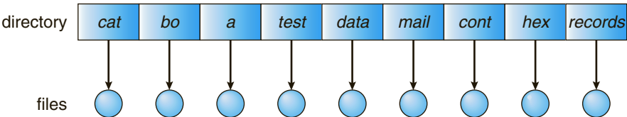
Figure 10.9 Single-level directory.
