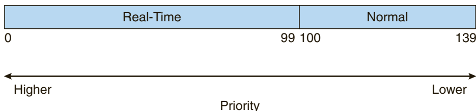
Figure 5.21 Scheduling priorities on a Linux system.
